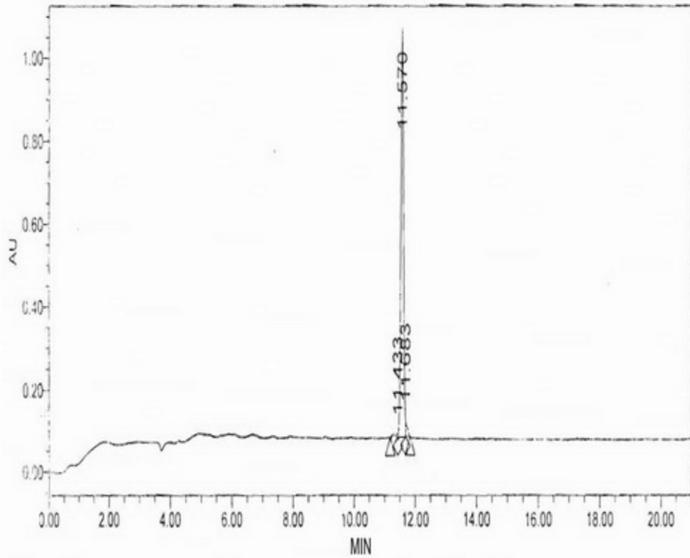
Figure. MASS Spectrometry.
