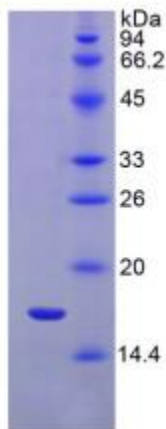
SDS-PAGE Image
