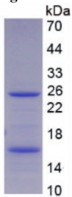
Figure. SDS-PAGE
