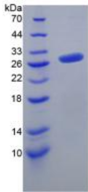
SDS-PAGE Image
