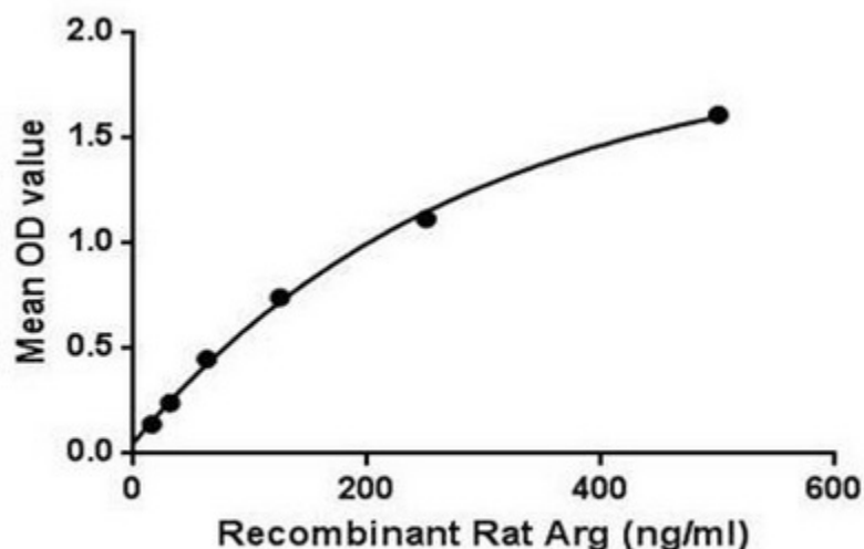
Figure 1. The binding activity of Arg with ERA.
