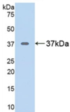
Figure. Western Blot; Sample: Recombinant Arg, Rat.
