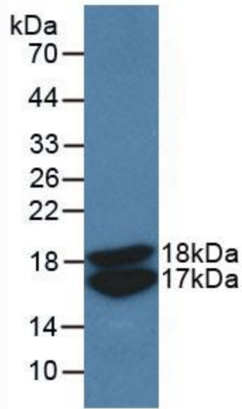
Figure. Western Blot; Sample: Recombinant VEGF121, Human.
