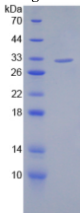
Figure. SDS-PAGE
