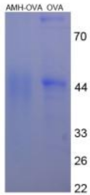
Figure. SDS-PAGE
