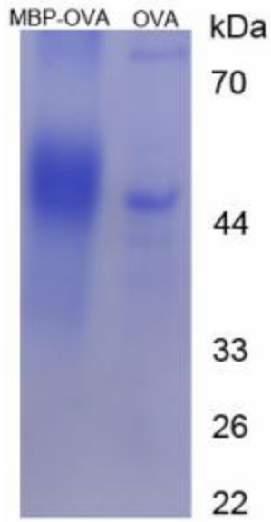
SDS-PAGE Image
