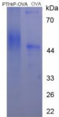
SDS-PAGE Image
