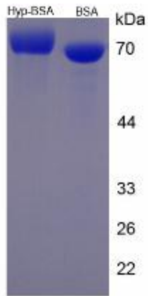
SDS-PAGE Image
