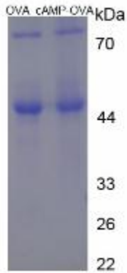
SDS-PAGE Image
