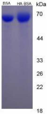
SDS-PAGE Image
