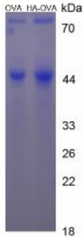
SDS-PAGE Image
