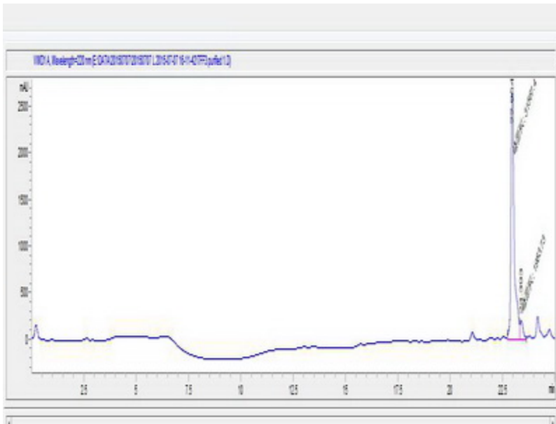
SDS-PAGE Image
