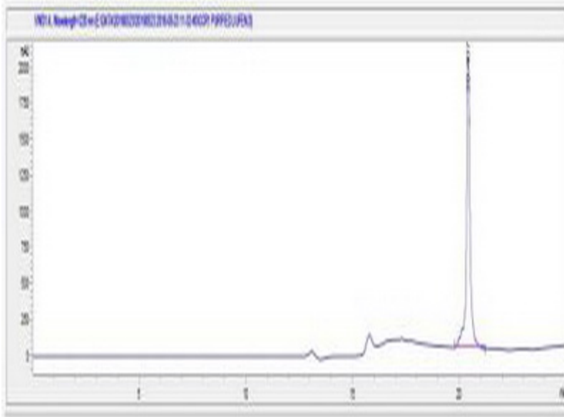
SDS-PAGE Image
