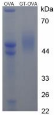
SDS-PAGE Image
