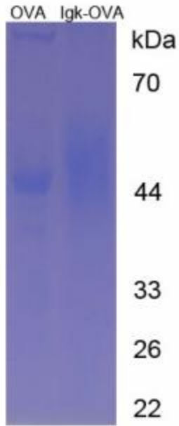
SDS-PAGE Image
