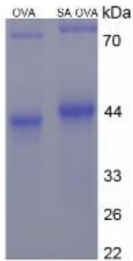
SDS-PAGE Image
