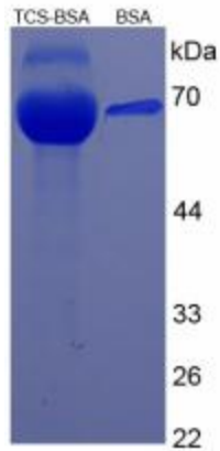
SDS-PAGE Image
