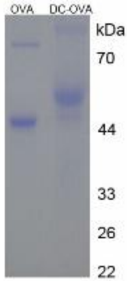
SDS-PAGE Image
