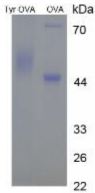
SDS-PAGE Image
