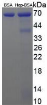
Figure. SDS-PAGE
