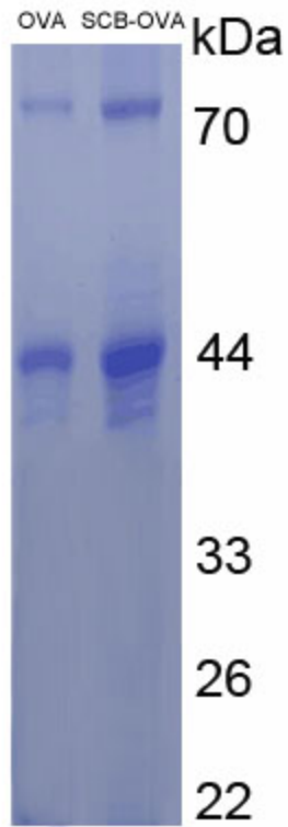
SDS-PAGE Image
