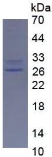
SDS-PAGE Image
