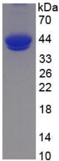
Figure. SDS-PAGE
