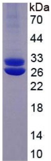
Figure. SDS-PAGE
