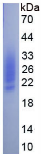
Figure. SDS-PAGE
