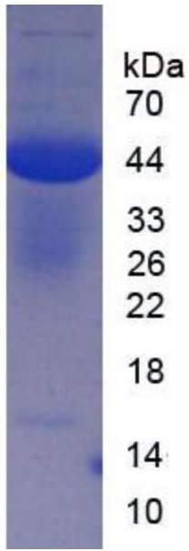
SDS-PAGE Image
