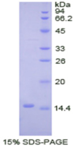
SDS-PAGE Image
