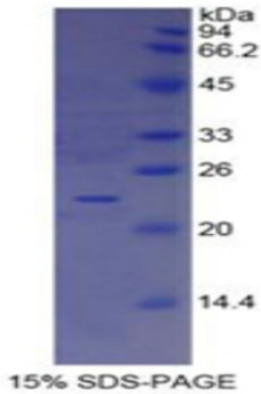
SDS-PAGE Image
