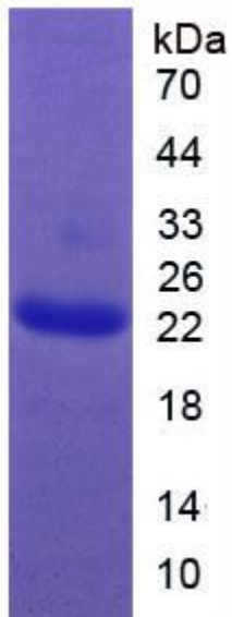
Figure. SDS-PAGE
