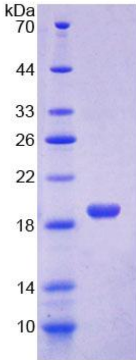
SDS-PAGE Image
