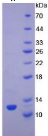
Figure. SDS-PAGE
