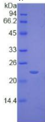
SDS-PAGE Image
