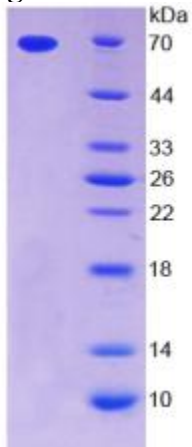
SDS-PAGE Image
