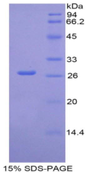
SDS-PAGE Image
