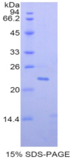
SDS-PAGE Image
