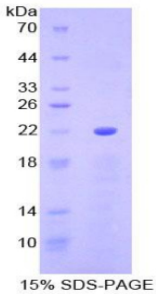
SDS-PAGE Image
