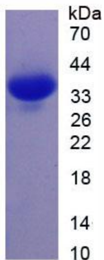
Figure. SDS-PAGE
