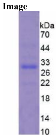
Figure. SDS-PAGE
