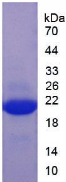
SDS-PAGE Image
