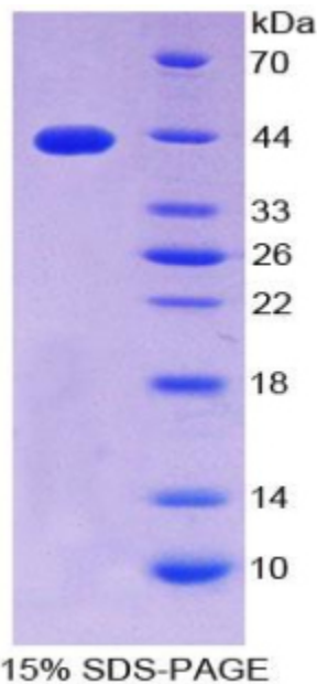
SDS-PAGE Image
