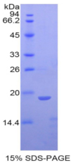
SDS-PAGE Image
