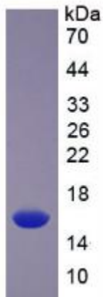
Figure. SDS-PAGE
