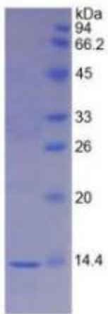
SDS-PAGE Image
