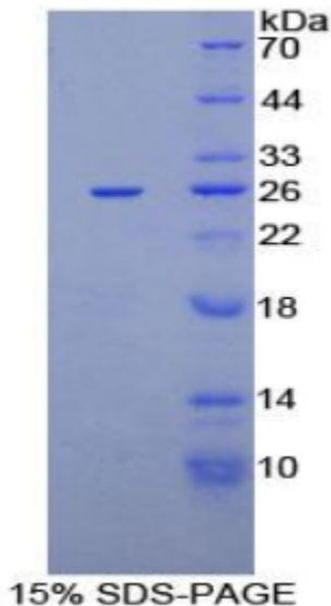
SDS-PAGE Image
