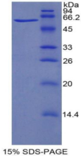
SDS-PAGE Image
