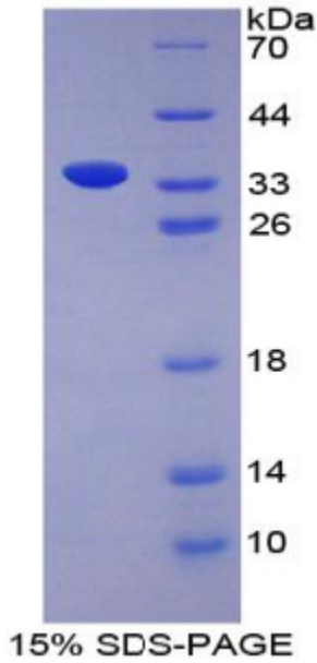
SDS-PAGE Image
