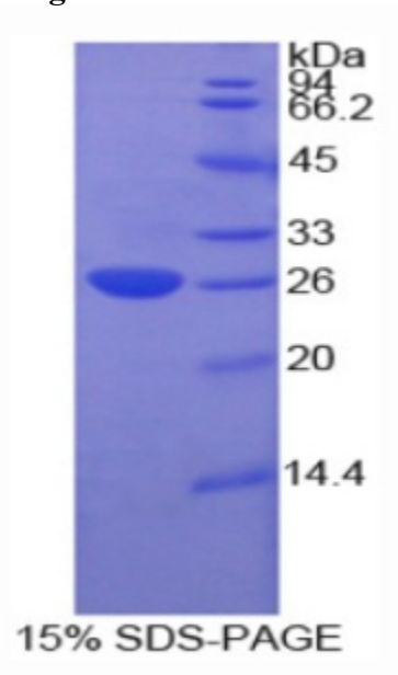
SDS-PAGE Image
